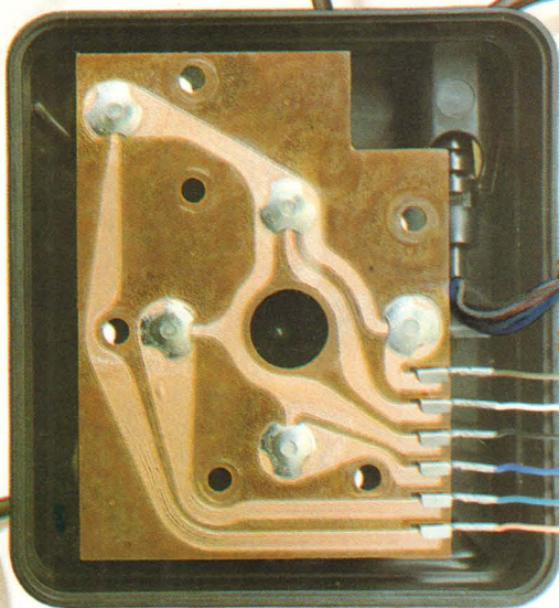
ORIGINAL WIRING
