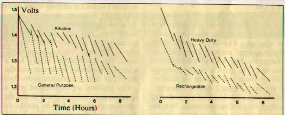
Figure 2. Discharge curves showing drop during use and recovery.
