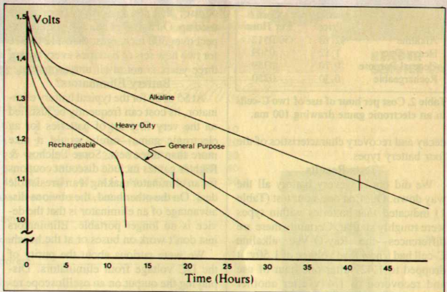
Figure 1. Discharge curves.
