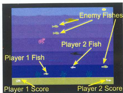
Figure 3. Two-player game.
