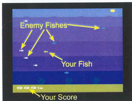
Figure 2. One-player game.
